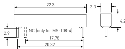
MK with integrated resistor
