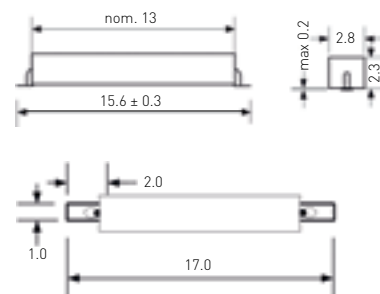
PMC-1001FH
