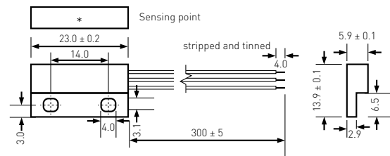
TS-324R
