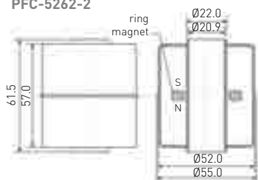
PFC-5262-2
