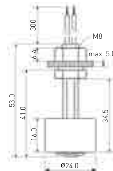
PLS-041 – Standard
