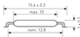
PMC-1001F
