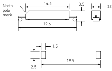
PMC-1001THY
